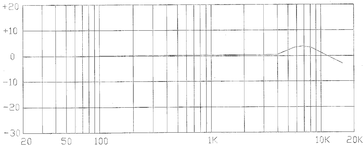
Frequency Response
