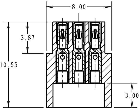
SECTION X-X
